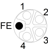
Figure 7: Schematic diagram of the M12 L-coding (socket X04 for Power Out)
