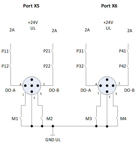
Figure 19: Schematic illustration of the DO functionality
