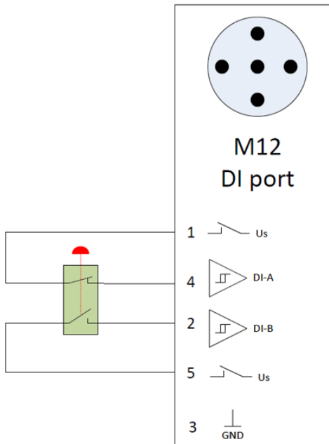
Figure 17: Internal SDI block diagram
