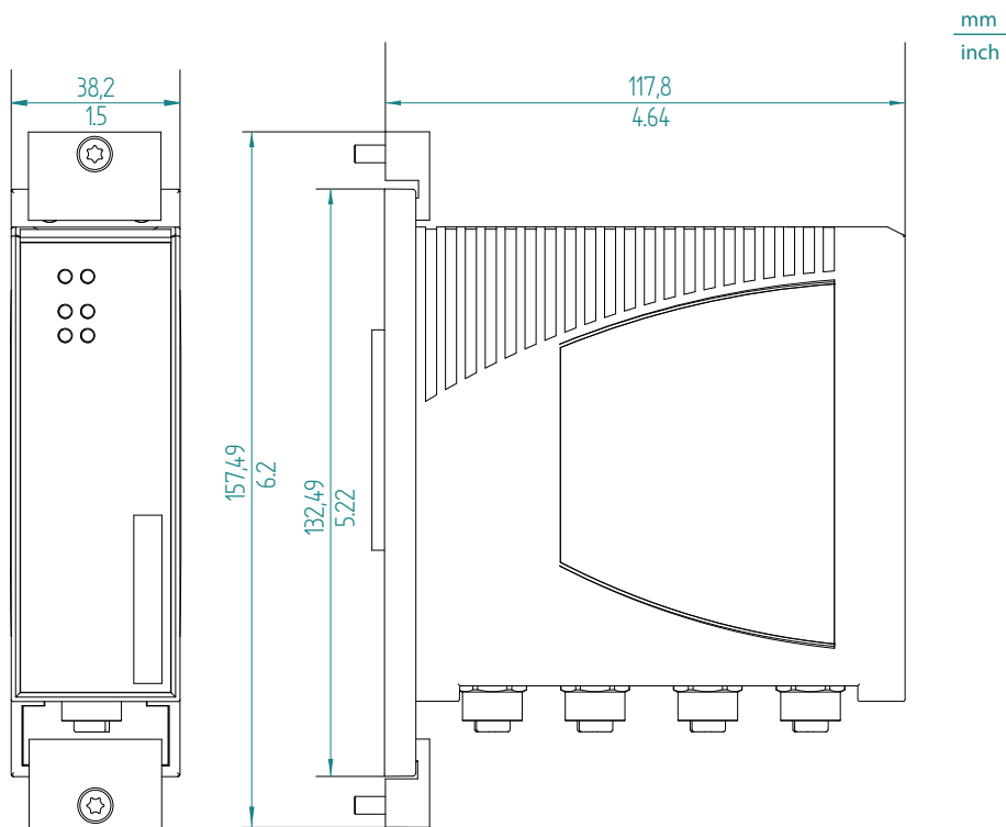
Figure 22: Dimensions for media modules with customer-specific version characteristic value HX
