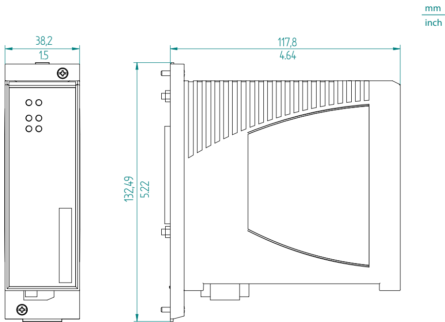
Figure 21: Dimensions for media module MSM46-T1T1T1T1... with characteristic value HH (with terminal block for external PoE supply voltage)
