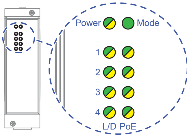
Figure 3: MSM22, MSM42 and MSM46 media modules: display elements (front view)
