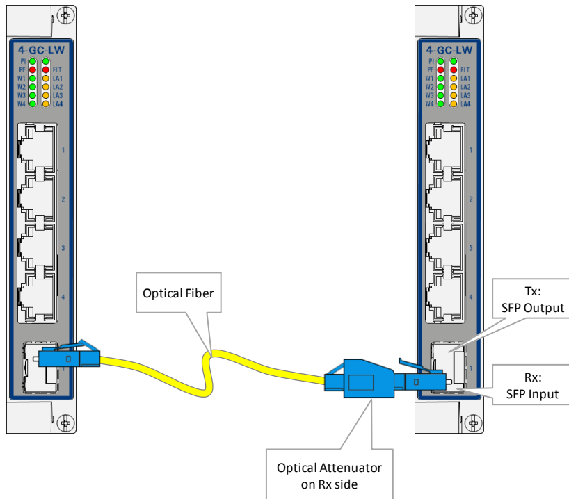
Figure 4 Optical Attenuator on Rx Side
