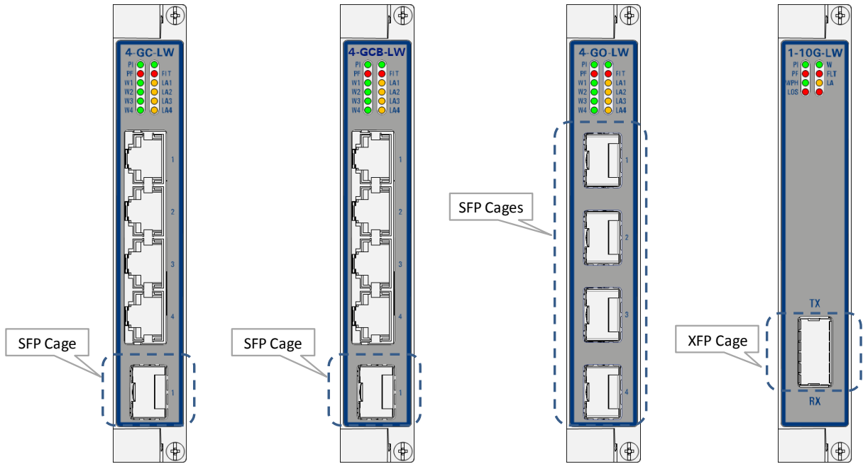
Figure 3 SFP/XFP Cages
