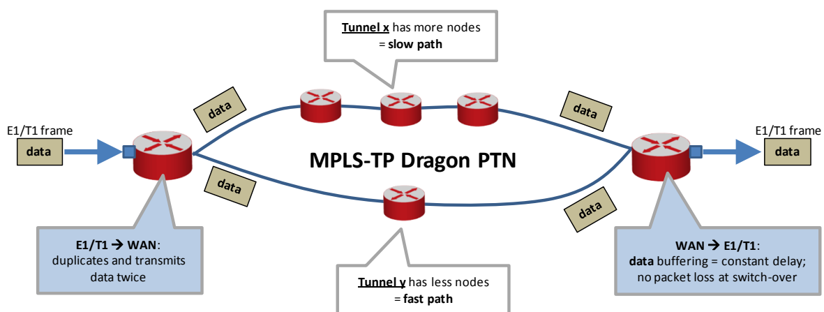
Figure 19 Hitless Switching
