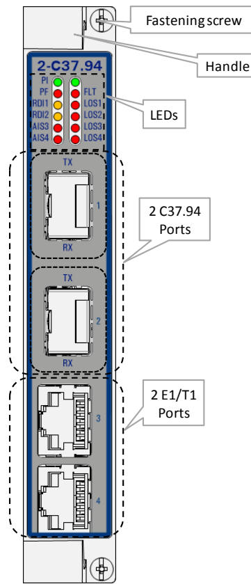
Figure 2 Front Panel
