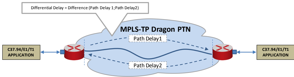
Figure 29 Differential Delay
