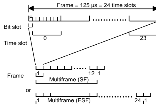
Figure 7 T1 Framing
