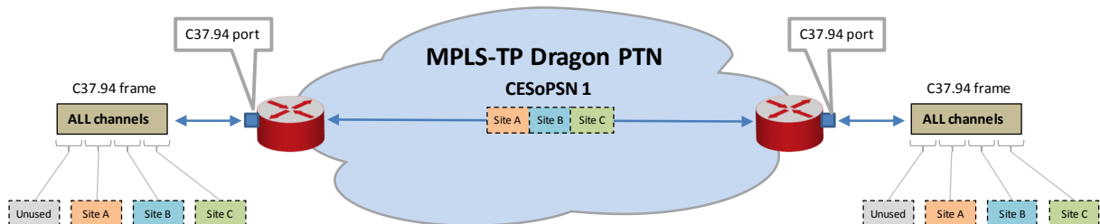
Figure 13 General CESoPSN via C37.94 Port Example
